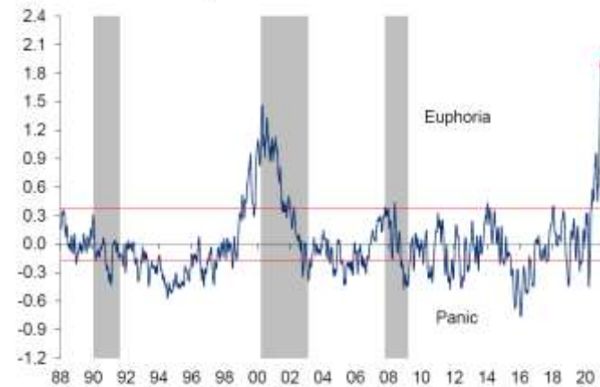
Figure 8. The Panic/Euphoria
